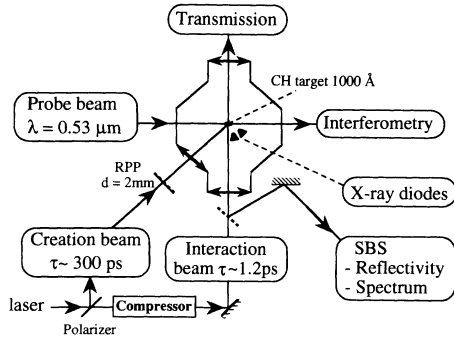
FIG. 1. Experimental setup.
