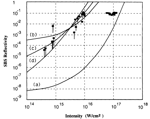
FIG. 2. Time-integrated SBS reflectivity, as a function of the laser intensity. The squares represent the experimental data and the solid lines represent the theoretical curves calculated for different noises (in terms of Thomson reflectivity R^{\text{Thom}} ): curve (a) R^{\text{Thom}} = R_{\text{Therm}}^{\text{Thom}} = 7.02 \times 10^{-9} , curve (b) R^{\text{Thom}} = 3.32 \times 10^{-4} , curve (c) R^{\text{Thom}} = 1.03 \times 10^{-5} I_{14} and curve (d) R^{\text{Thom}} = 3.20 \times 10^{-7} I_{14}^2 . The parameters are L = 600\ \mu\text{m} , T_e = 0.1 keV, T_i = 0.06 keV, and n_e/n_c = 0.04 .
