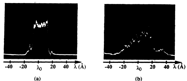
FIG. 3. Incident (a) and reflected (b) spectra for a laser intensity of 10^{17} W/cm 2 .
